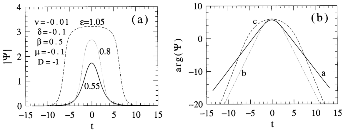
Figure 2. Stable pulse solutions of the CGLE obtained numerically using parameters as indicated, in the normal dispersion regime. (a) Amplitude profile. (b) Phase profile. The three pulse profiles are obtained by varying the nonlinear gain parameter \varepsilon . After [43].
