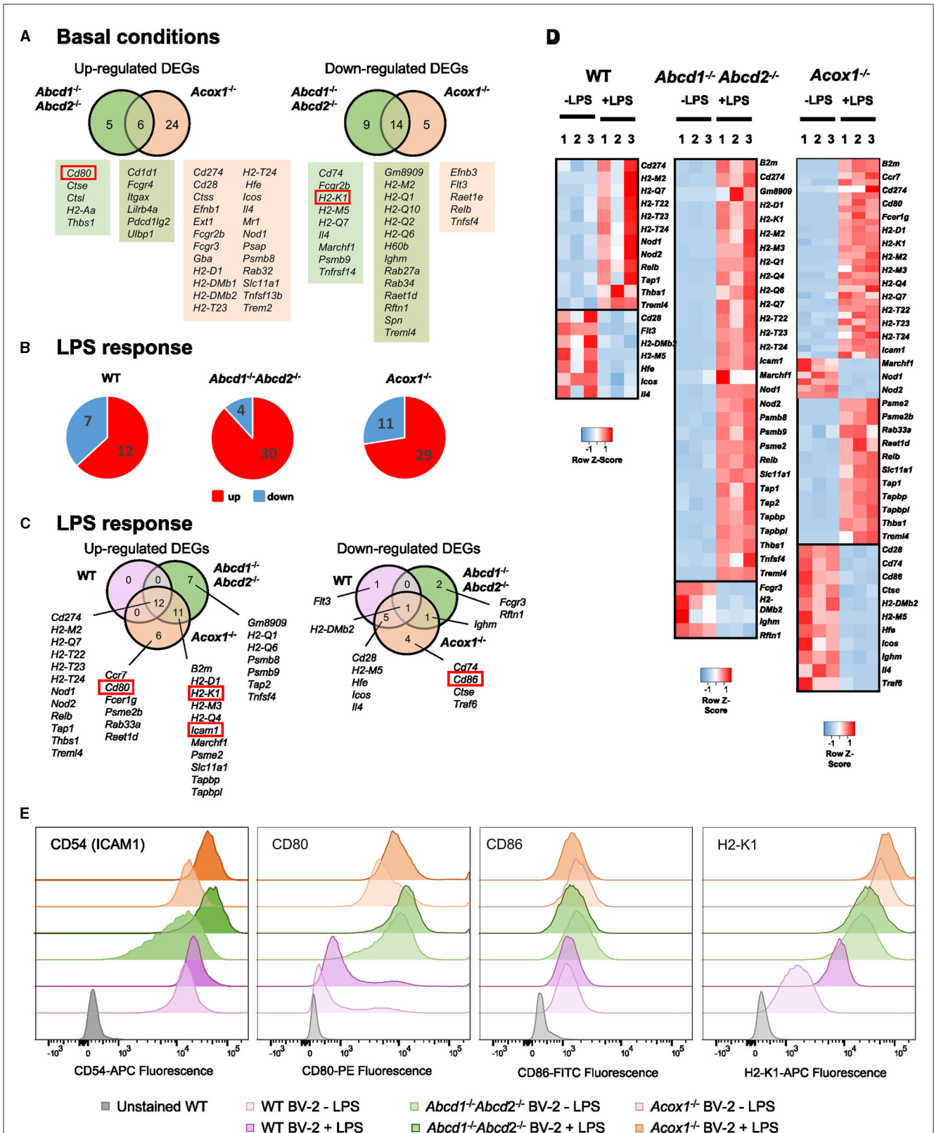
FIGURE 5 Impact of peroxisomal defect on the expression of genes related to antigen presentation and T lymphocyte co-stimulation in WT and mutant ( Abcd1 -/- Abcd2 -/- and Acox1 -/- ) BV-2 cells. (A) Venn diagrams illustrating the up- and downregulated DEGs (Log2FC > 1, AdjP Value < 0.05) related to antigen presentation and T lymphocyte co-stimulation in Abcd1 -/- Abcd2 -/- and Acox1 -/- non-stimulated BV-2 cells (DataSet GSE200022). Genes whose expression level was measured at the protein level are boxed. (B) Pie chart displaying the number of these up- or downregulated DEGs after a 24-h LPS treatment (Log2FC > 1, AdjP Value < 0.05) in WT, Abcd1 -/- Abcd2 -/- , and Acox1 -/- BV-2 cells (DataSet GSE237635). (C) Venn diagrams representing the LPS response in each genotype of these DEGs (three independent batches of BV-2 cells for each genotype). (D) Heat map representing RNA-Seq gene expression (with Z-scores) of these DEGs at 24 h after LPS stimulation in WT, (Continued)
