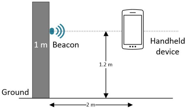
Fig. 17. Mounting a beacon at 1.2m-height
