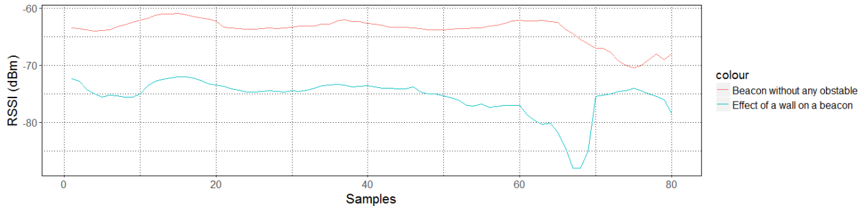
Fig. 20. RSSI plot to see the effect of a building obstacle (i.e. wall) on beacon
