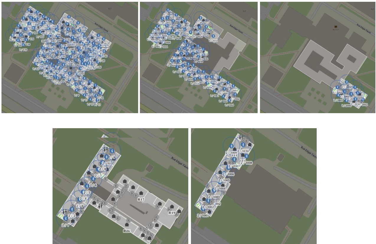
Fig. 3. Deployment maps of BLE beacons of different floors in two buildings
