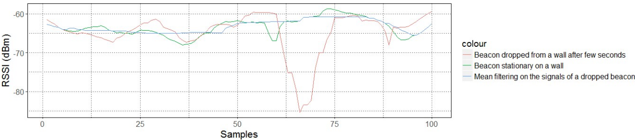
Fig. 18. Effect of falling off a beacon
