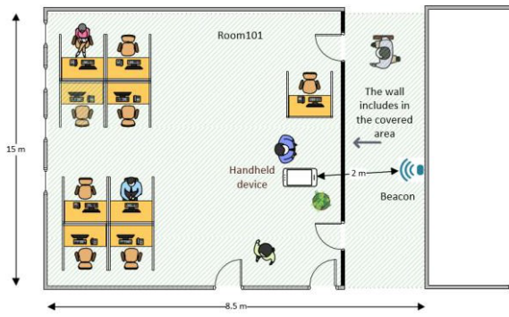
Fig. 19 (b) Effect of a wall on RSSI of a beacon
